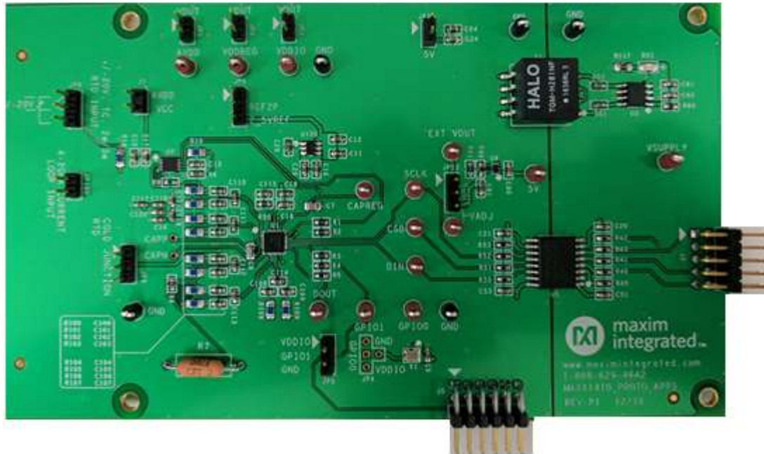
Figure 1: AFE Board (Sensor Front End, Switch, Passives, ADC, Reference, Reference Power Supply, Isolated Supply, Data Isolator)
